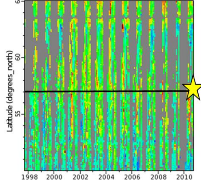
Chlorophyll-a, Orbview-2 SeaWiFS, R2018.0, 0.1°, Global, 1997-2010 (Monthly Composite)
