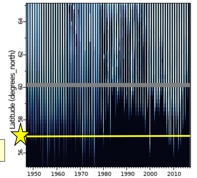
Sea Ice Extent and Concentration V2, NOAA/NSIDC, Arctic, 25km, 1850+, Mo
