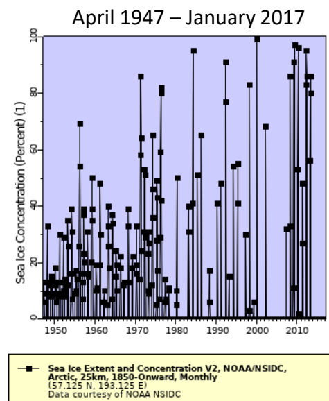
Sea Ice Extent and Concentration V2, NOAA/NSIDC, Arctic, 25km, 1850+, Mo
