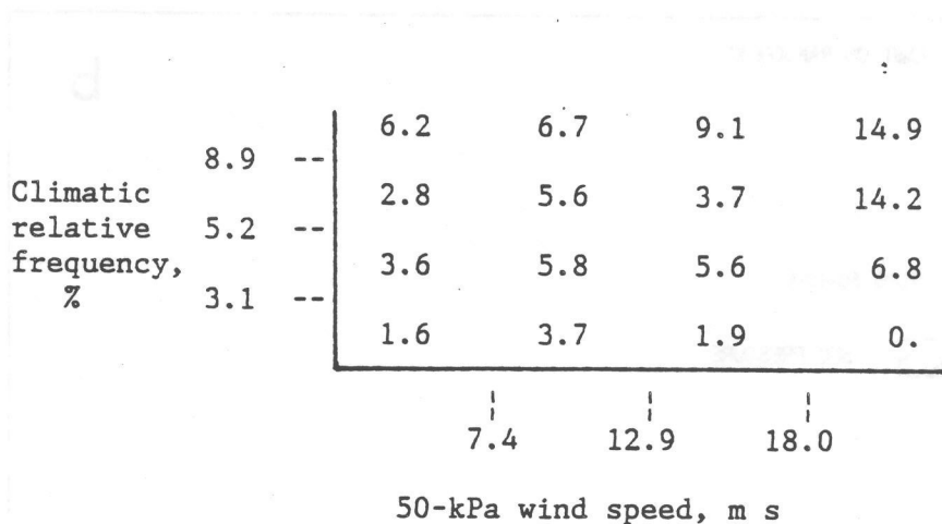
Figure 13. Conditional severe local storm relative frequency, per cent, as a function of climatic relative frequency (vertical coordinate) and 50-kPa wind speed (horizontal coordinate). Wind speed is derived from 1700 GMT VAS retrievals; climatic frequency based on 1974-1983 severe storm reports. Observation period is 2000-0000 GMT.
