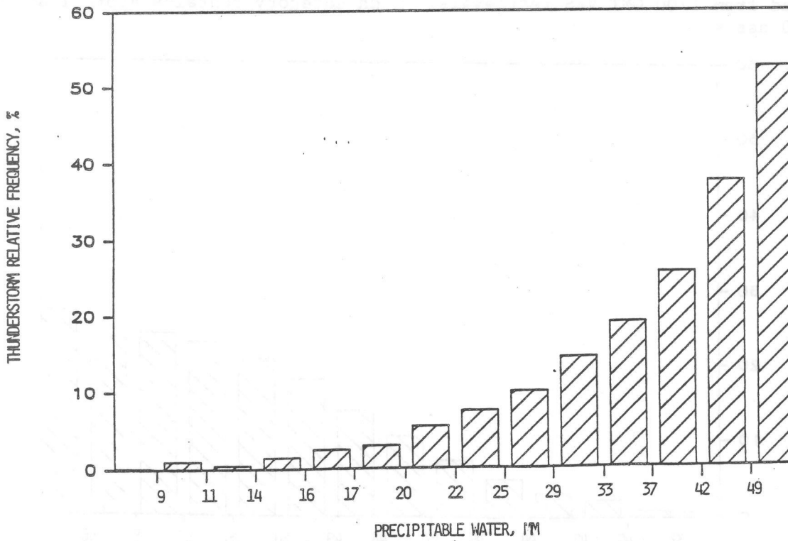
Figure 5. As in Fig. 1, except predictor is precipitable water (PW).
