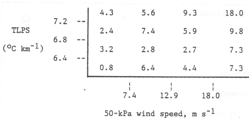
Figure 12. Conditional severe local storm relative frequency, percent, as a function of TLPS (vertical coordinate) and 50-kPa wind speed (horizontal coordinate). Predictors are derived from 1700 GMT VAS retrievals; observation period is 2000-0000 GMT.
