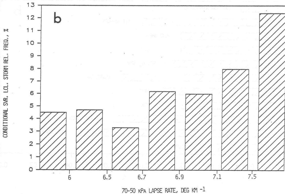
Figure 10. Observed severe local storm relative frequency within thunderstorm cases as a function of (a) 50-kPa wind speed, and (b) 70-50 kPa temperature lapse rate (TLPS). Storm events occurred during the period 2000-0000 GMT; predictors were derived from 1700 GMT VAS retrievals. Each category includes approximately 460 events.
