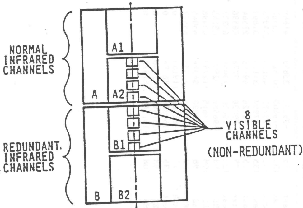
Figure 1. The configuration of the imager detectors of GOES I through M reproduced from Integral Systems (1988).
