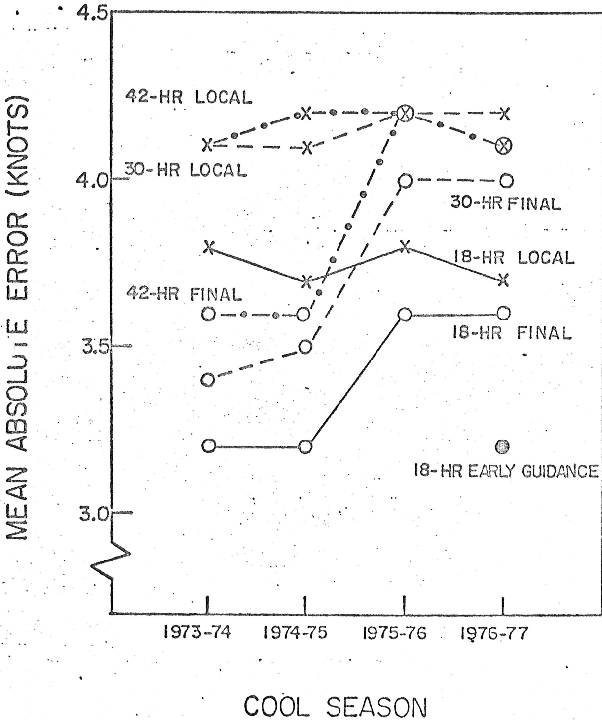
Figure 4.2 Same as Figure 4.1 except for wind speed forecasts.
