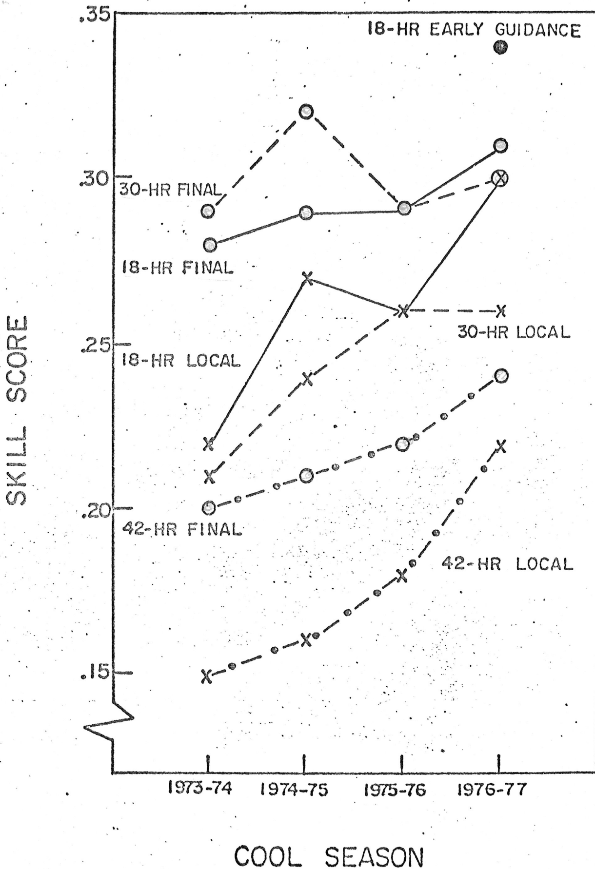
Figure 4.3. Skill scores for subjective local and objective guidance (early and final) surface wind speed forecasts for approximately 90 U.S. stations.
