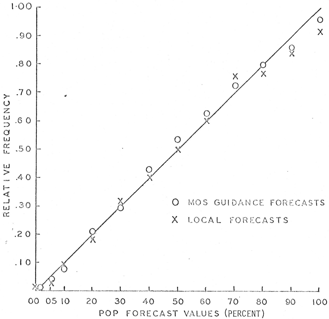
Figure 2.1 Reliability of final guidance and local PoP forecasts.
