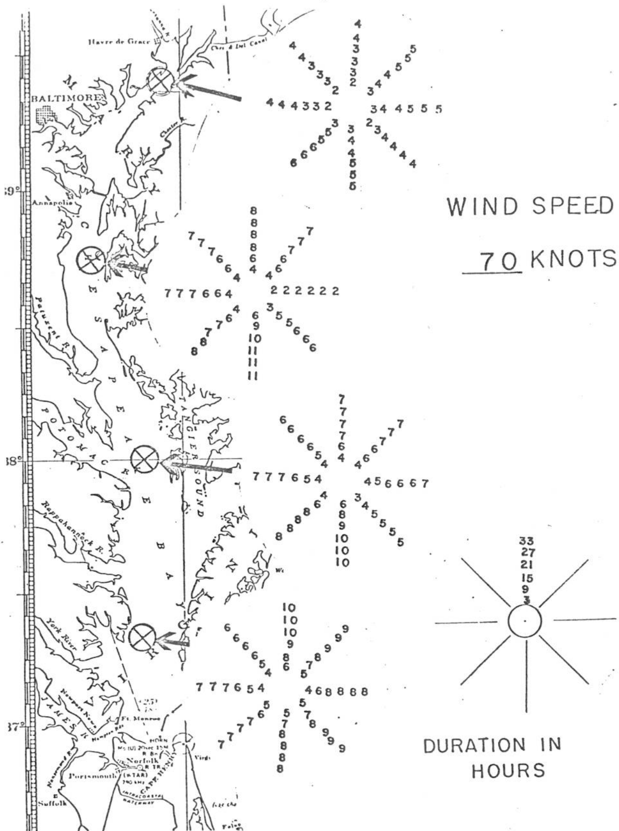
Figure 15. Significant wave heights at four points for wind of 70 knots from eight directions. For each direction wave heights are presented for wind durations of 3, 9, 15, 21, 27, and 33 hours. Wave heights are shown in feet.
