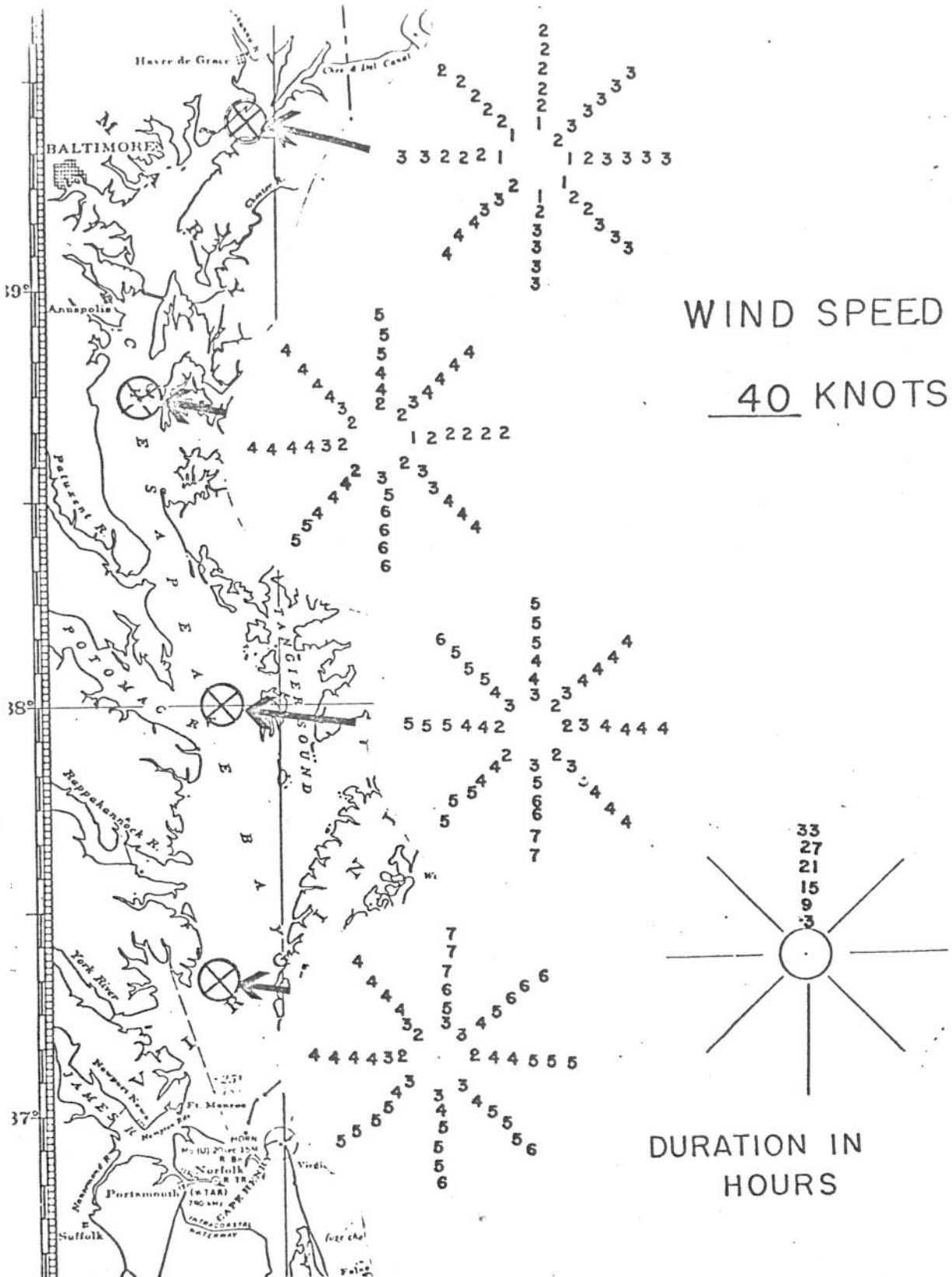
Figure 9 . Significant wave heights at four points for wind of 40 knots from eight directions. For each direction wave heights are presented for wind durations of 3, 9, 15, 21, 27, and 33 hours. Wave heights are shown in feet.
