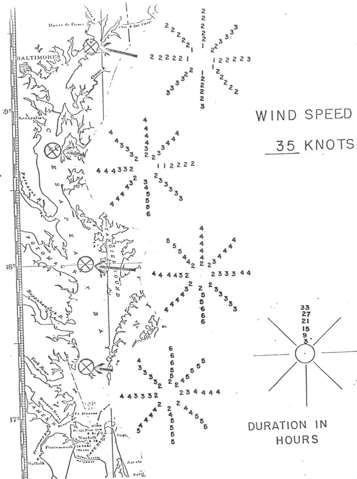
Figure 8 . Significant wave heights at four points for wind of 35 knots from eight directions. For each direction wave heights are presented for wind durations of 3, 9, 15, 21, 27, and 33 hours. Wave heights are shown in feet.
