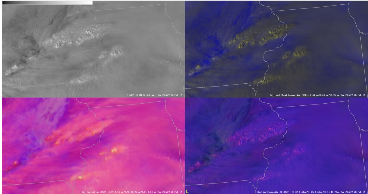
Figure 5. GOES-16 Satellite Imagery 4-Panel from 28 February 2017 at 21:22 UTC. Top left panel is the “Red” Band Visible, top right panel is the Day Land Cloud Convection RGB, bottom left panel is the Day Convection RGB, and the bottom right panel is the Daytime Composite #1 RGB.
