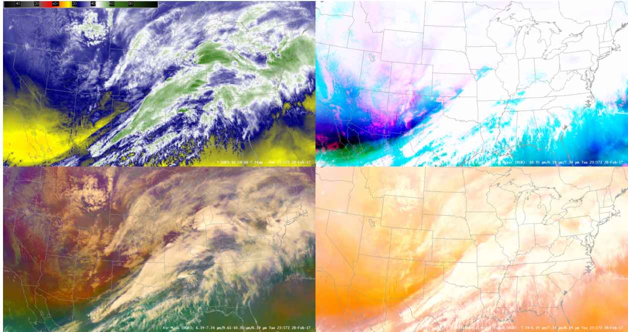
Figure 6. GOES-16 Satellite Imagery 4-Panel from 28 February 2017 at 23:57 UTC. Top left panel is the “Lower-Level Water Vapor” Band IR, top right panel is the Simple Water Vapor RGB, bottom left panel is the Air Mass RGB, and the bottom right panel is the Differential Water Vapor RGB.
