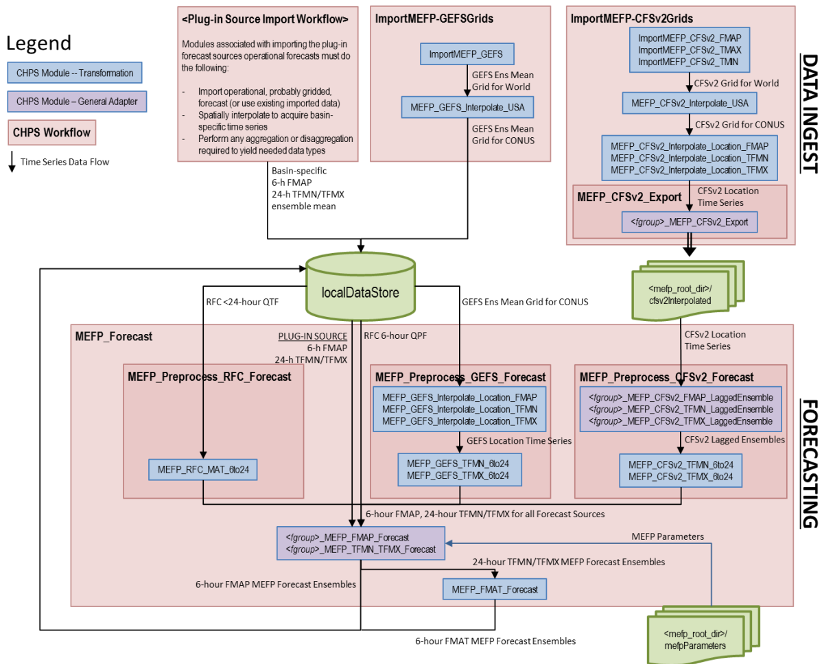
Figure 2: Diagram of the CHPS modules that are part of the MEFP data ingest and forecasting components.
