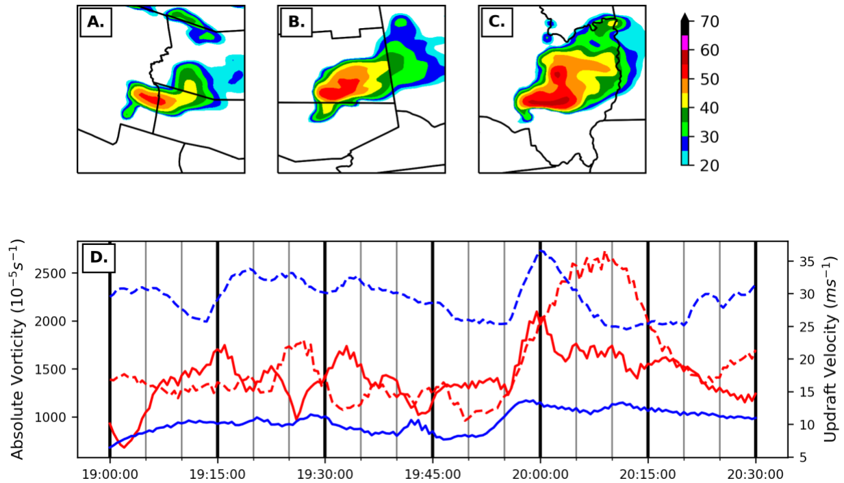
Figure 2. Simulated radar reflectivity (dBZ) for the Mechanicville supercell at (a) 1900, (b) 1930, and (c) 2000 UTC 31 May 1998. (d) Maximum 1-km updraft (blue, solid), 5-km updraft (blue, dashed), 1-km absolute vorticity (red, solid), and 5-km absolute vorticity (red, dashed). The supercell crosses a terrain-induced boundary around 1945 UTC and intensifies shortly after.
